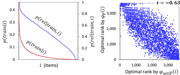
Figure 3: Comparison of the popularity and average rating distributions over items in MovieLens 1M (left), and how this results in an opposing trend between the optimal rankings for observed precision and anti-precision (right). The curves in the left graph are sorted in decreasing order of p(\text{train}|i) and p(\text{rel}|\text{train}, i) respectively (hence the x axis is ordered differently for each curve). Each dot in the right plot is an item, and its coordinates reflect its rank in the corresponding optimal ranking. The Kendall \tau correlation between the rankings is shown.
